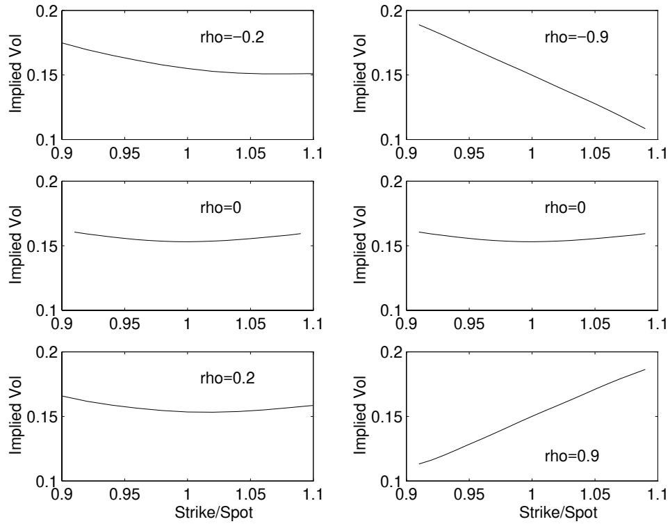
Figure 1: Simulated Smile Curves for Options with Maturity of 120 days. The Volatility of Volatility, V , is Fixed at 1 per annum; the Level of Correlations, \rho , varies from -0.9 to 0.9, as Marked in Each Plot.
