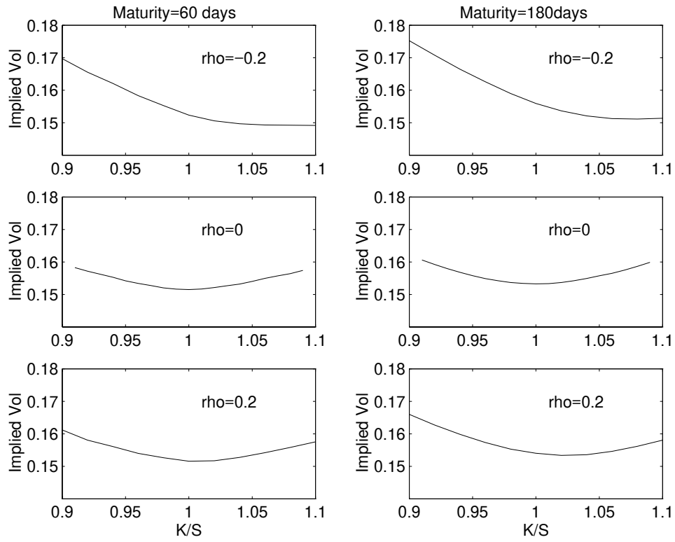
Figure 3: Simulated Smile Curves for Options with Maturity of 60 days and 180 days. The Volatility of Volatility, V , is Fixed at 1 per annum; the Level of Correlations, \rho takes value of \pm 0.2 as Marked in Each Plot.
