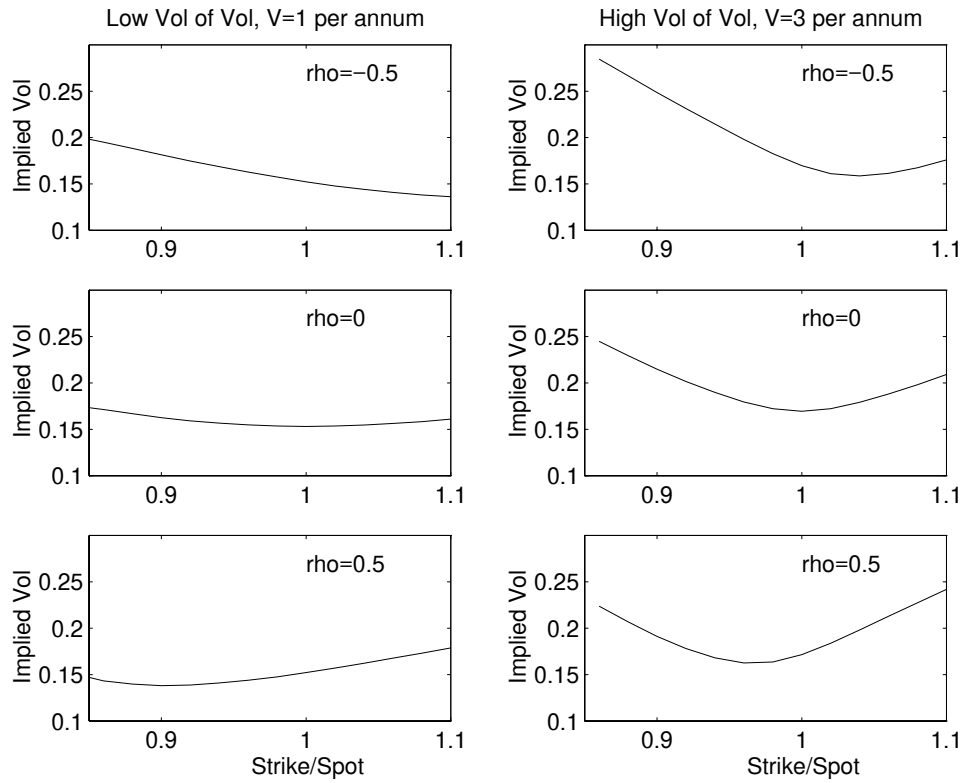
Figure 2: Simulated Smile Curves for Options with Maturity of 120 days. The Volatility of Volatility, V , is Fixed at 1 per annum for the Left Panels, and 3 per annum for the Right Panels; the Level of Correlations, \rho , varies from -0.5 to 0.5, as Marked in Each Plot.
