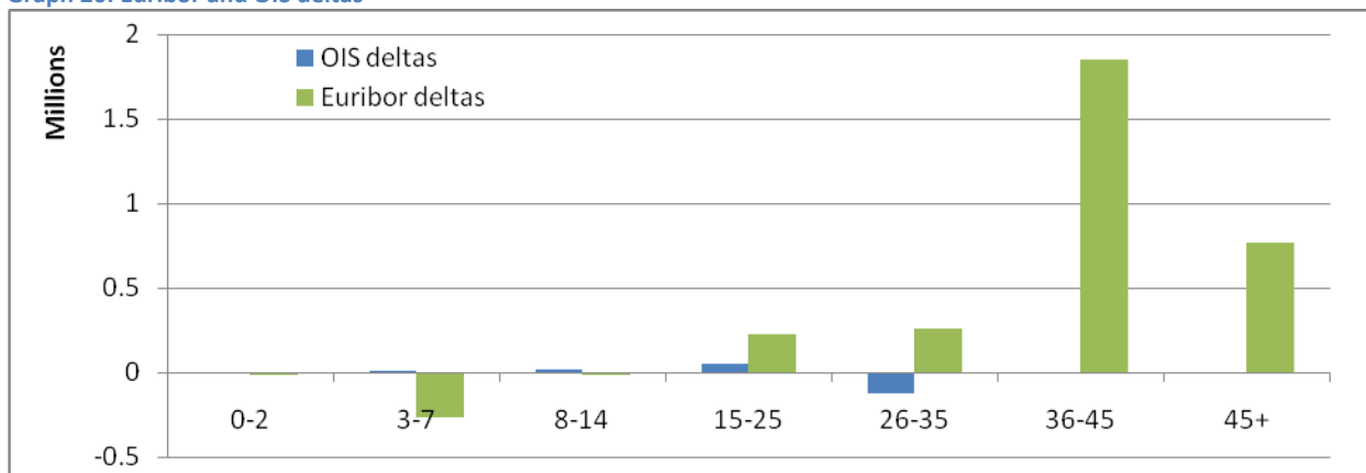
Graph 20: Euribor and OIS deltas
