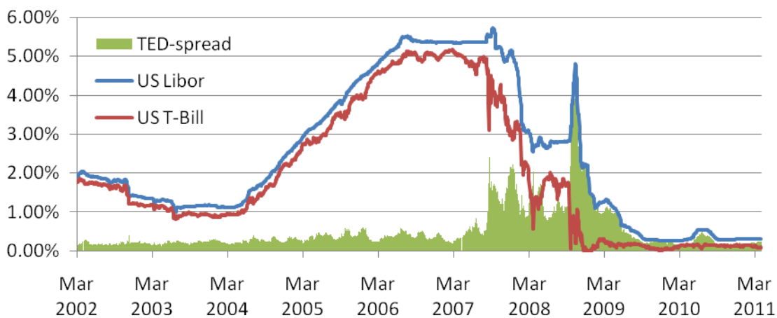
Graph 2: 3m US Libor versus 3m T-Bill: The TED spread
