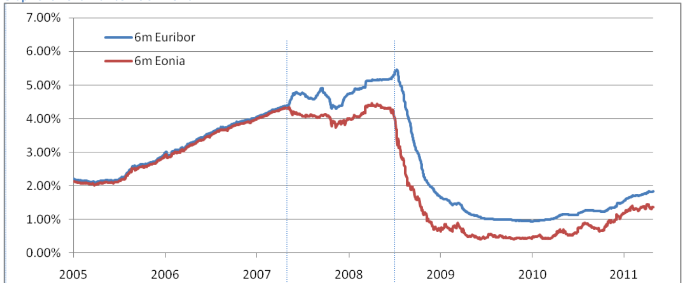
Graph 3: 6month Euribor vs 6m Eonia
