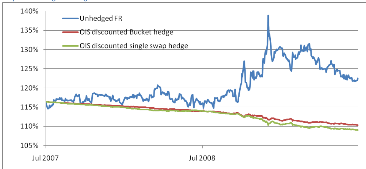
Graph 23: Unhedged vs hedged FR in simulated scenario
