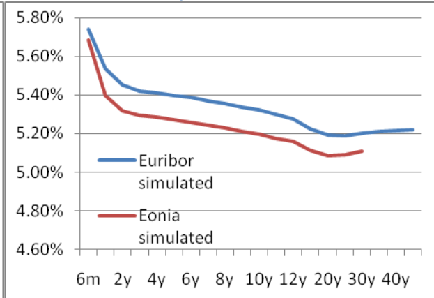
Simulated swap curves for robustness test.
