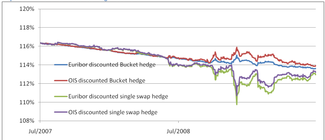
Graph 18: Eonia vs Euribor discounted hedge instruments
