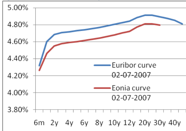
Figure 1: Euribor and Eonia swap curve on 02-07-2007
