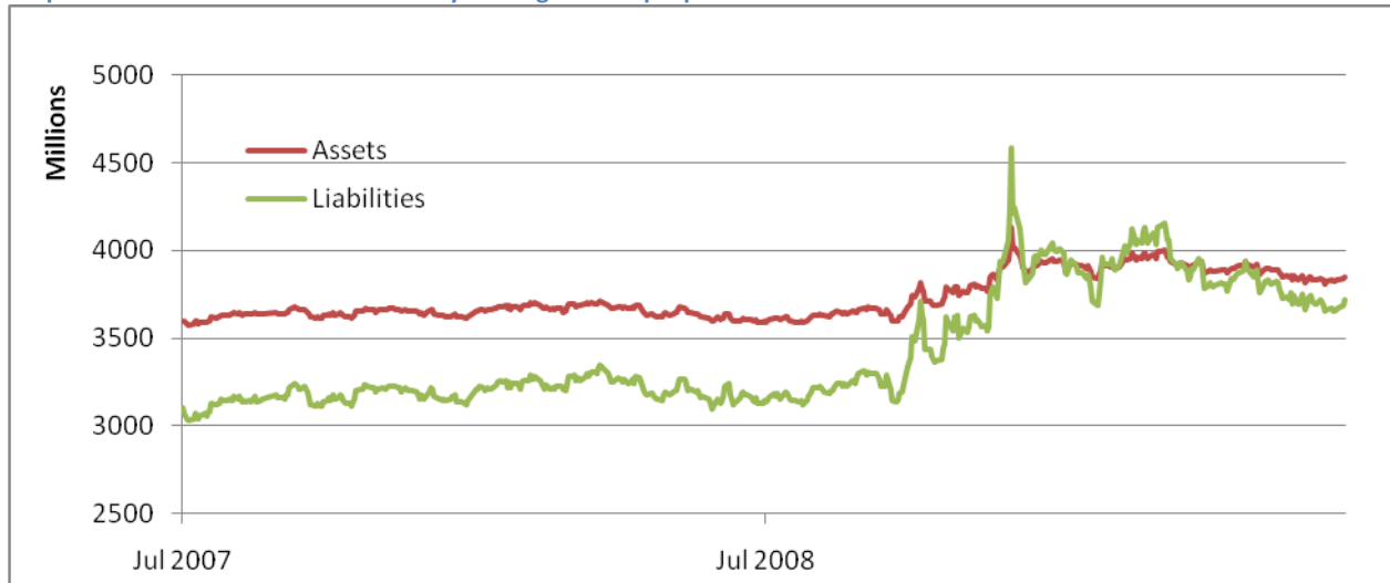
Graph 13: Assets and liabilities of fund xyz during the sample period
