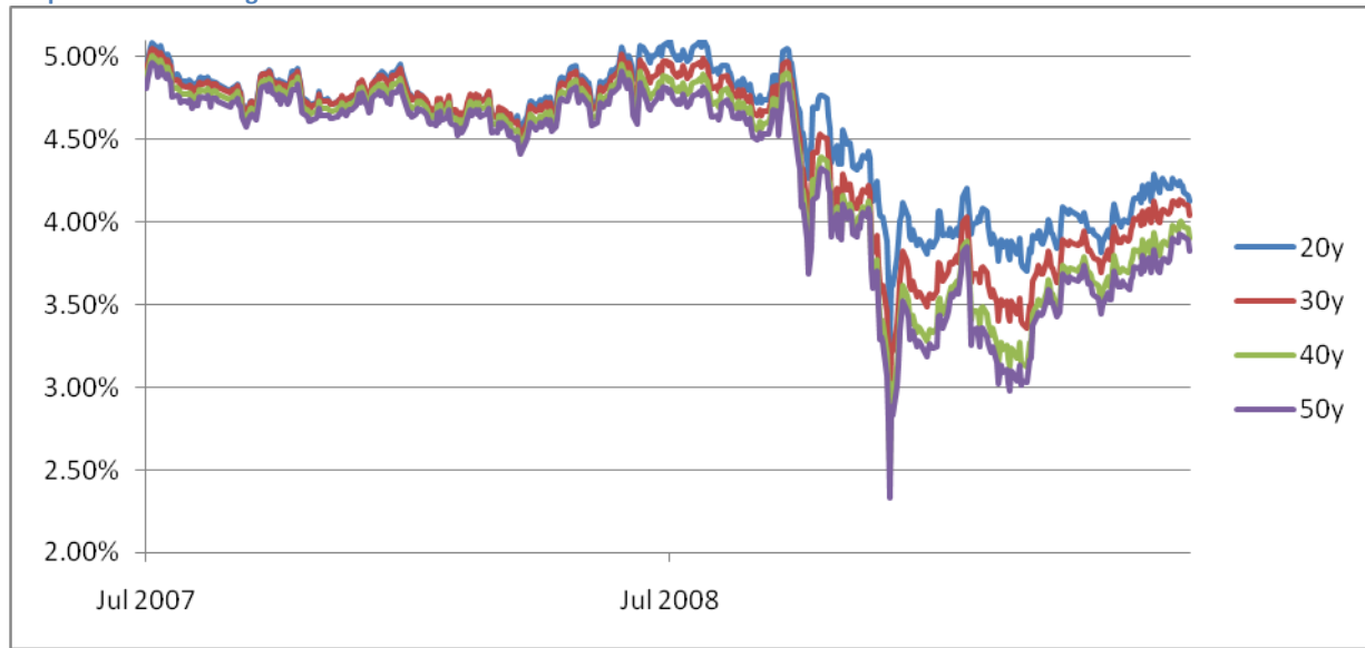
Graph 12: Euribor long interest rates
