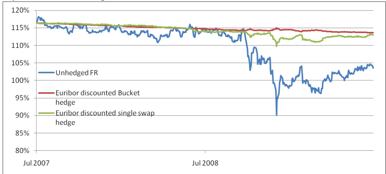
Graph 16: Euribor discounted hedged FRs
