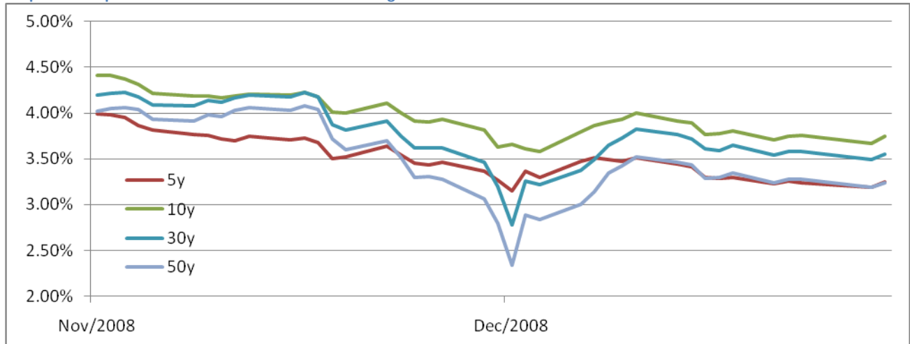
Graph 17: Swap rates of four Euribor instruments during November-December 2008
