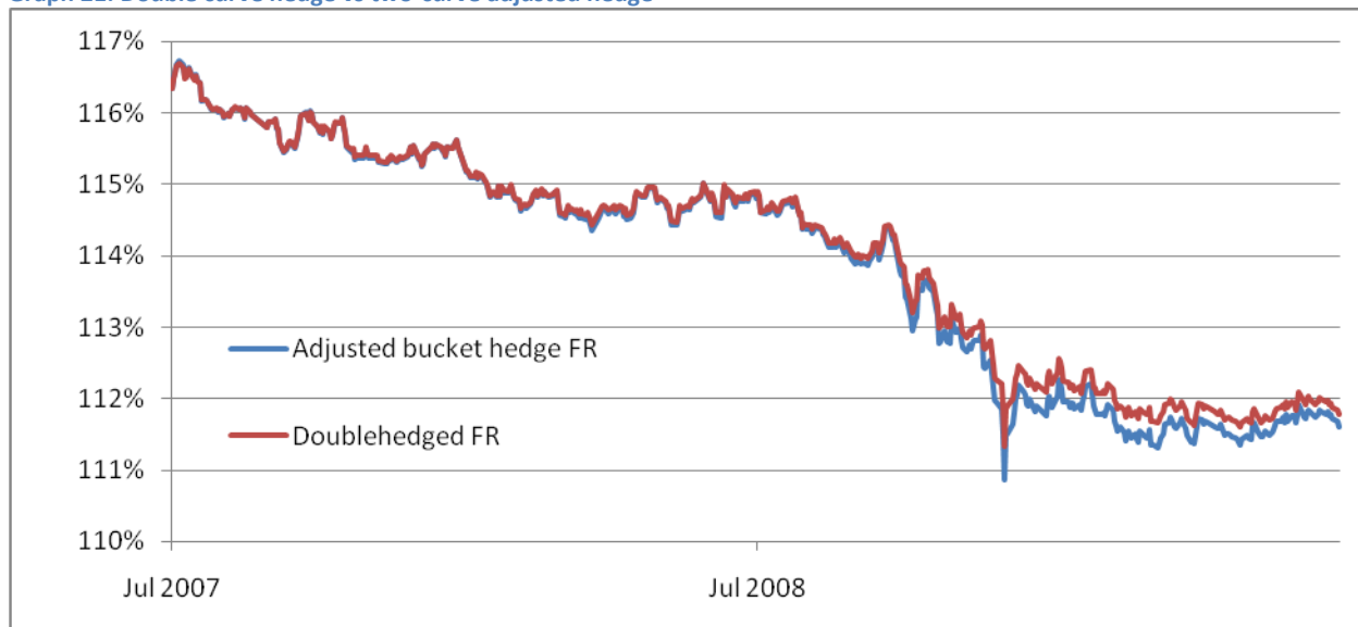
Graph 21: Double curve hedge vs two-curve adjusted hedge
