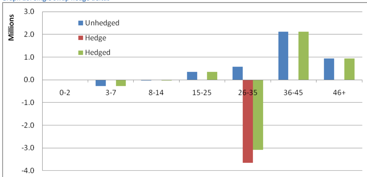
Graph 10: Single swap hedge deltas
