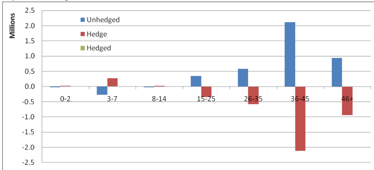
Graph 11: Bucket hedge deltas
