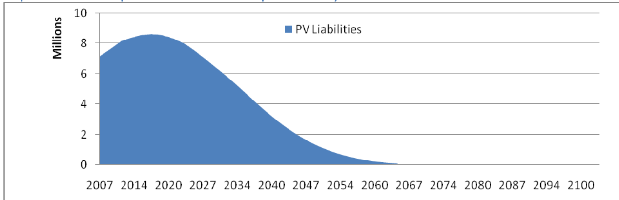
Graph 6: Distribution of present value of liabilities of pension fund xyz over time
