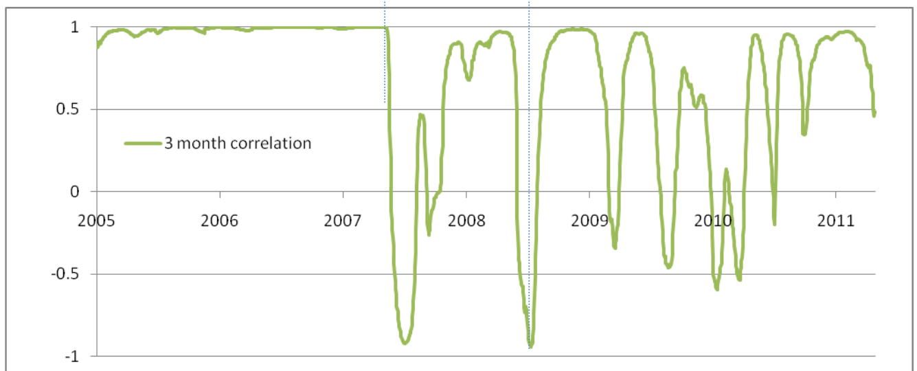
Graph 4: Correlation 6m Euribor with 6m Eonia (three month backwards rolling level average, so t-3m to t)
