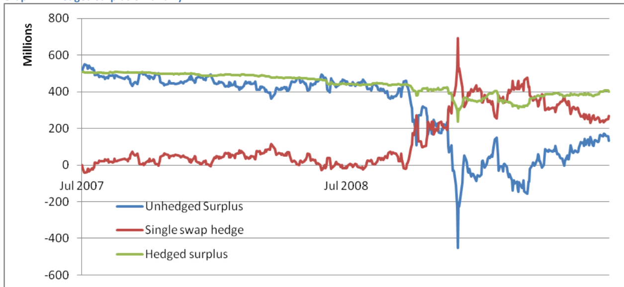
Graph 14: Hedged surplus of fund xyz
