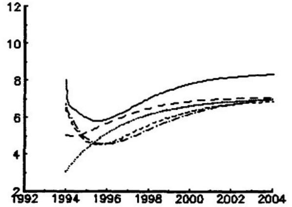
Figure 14. Forward Rates by Trade Date
