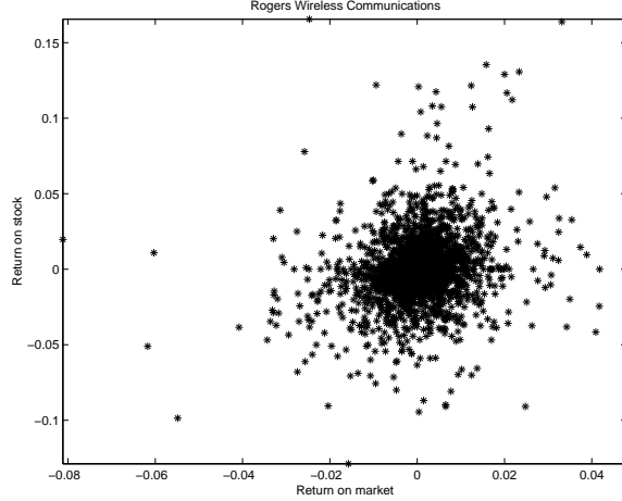
Figure 10.4: Return on Rogers Wireless Communications versus return on TSE 300. Each point represents pairs of daily returns. The vertical axis measures the daily return on the stock and the horizontal axis that of the TSE300.
