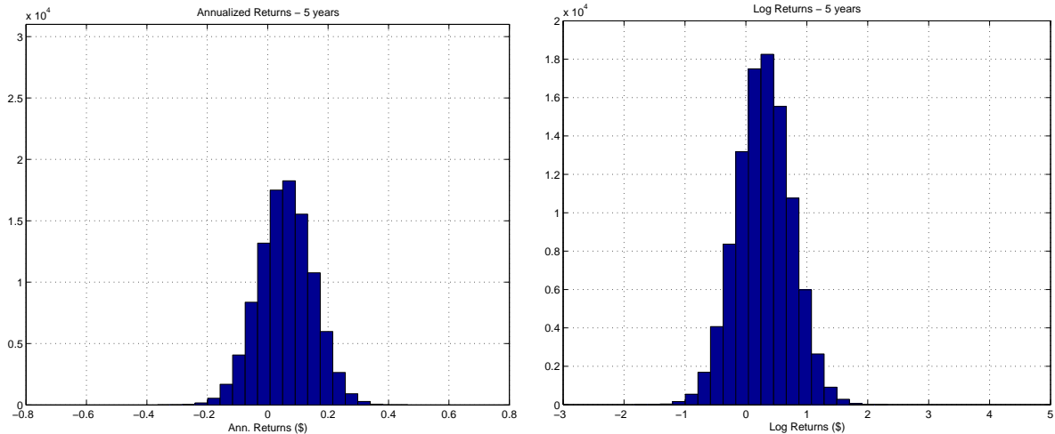
Figure 11.1: Histogram of distribution of returns T = 5 years. \mu = .08, \sigma = .2 , 100,000 simulations. Left: annualized return 1/T \log[S(T)/S(0)] . Right: return \log[S(T)/S(0)] .
