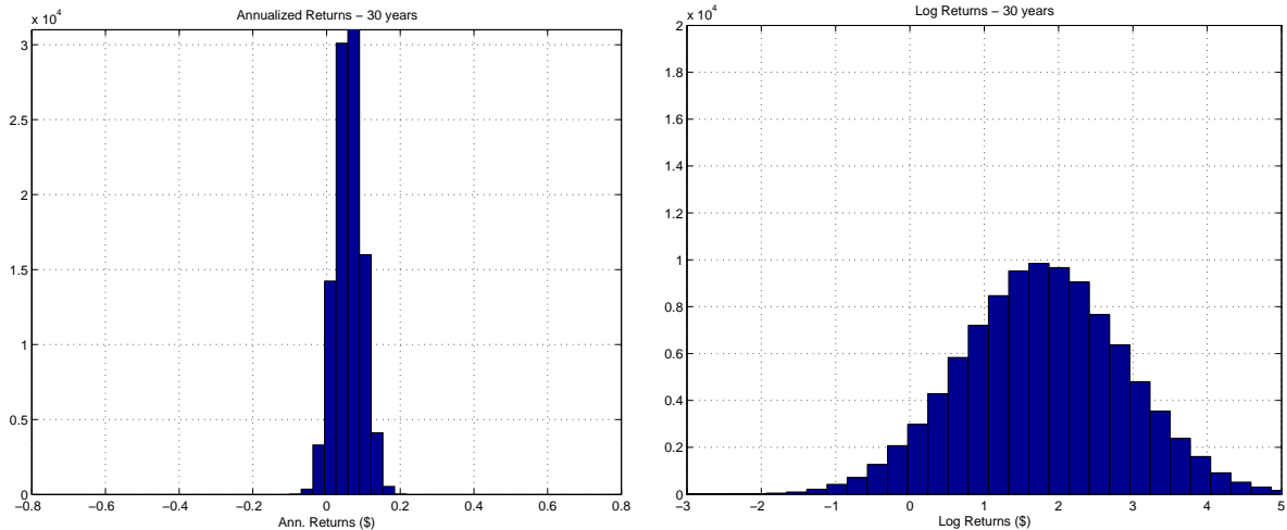
Figure 11.2: Histogram of distribution of returns T = 30 years. \mu = .08, \sigma = .2 , 100,000 simulations. Left: annualized return 1/T \log[S(T)/S(0)] . Right: return \log[S(T)/S(0)] ,
