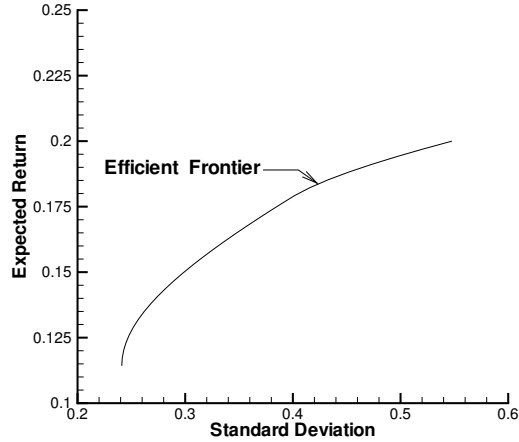
Figure 10.1: A typical efficient frontier. This curve shows, for each value of portfolio standard deviation SD(R_p) , the maximum possible expected portfolio return R_p . Data in equation (10.20).
