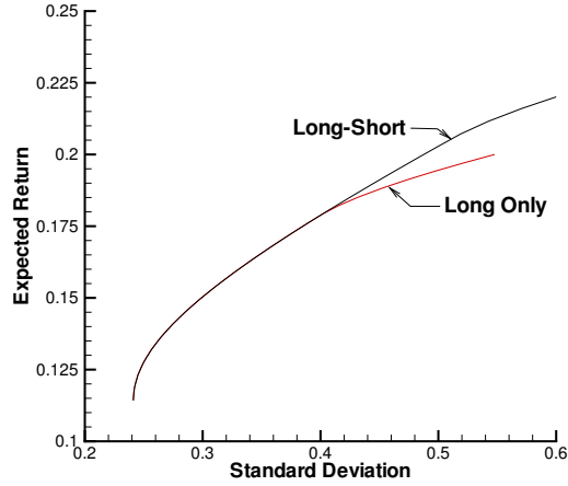
Figure 10.2: Efficient frontier, comparing results for long-only portfolio (10.20) and a long-short portfolio (same data except that lower bound constraint is replaced by equation (10.21)).
