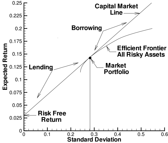
Figure 10.3: The efficient frontier from Figure 10.1 (all risky assets), and the efficient frontier with the same assets as in Figure 10.1, except that we include a risk free asset. In this case, the efficient frontier becomes a straight line, shown as the capital market line.
