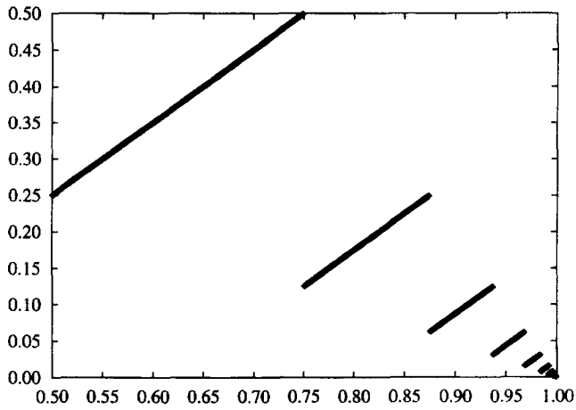
Fig. 4. 2000 one-dimensional Faure points.
