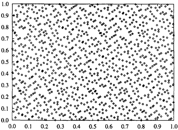
Fig. 3. 1000 two-dimensional Sobol's points.
