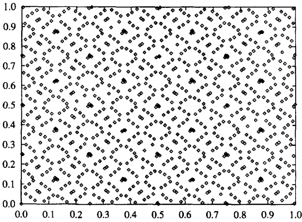
Fig. 2. 1000 two-dimensional Faure points.
