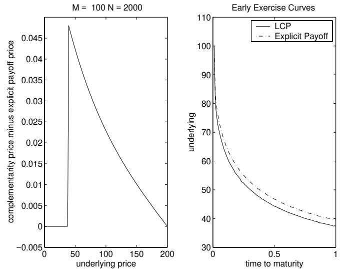
FIG. 1. LCP Comparisons : S_0 = 100 , K = 100 , T = 1 , r = 0.1 , q = 0 , \sigma = 0.8 , \epsilon_{opt} = 10^{-4}
