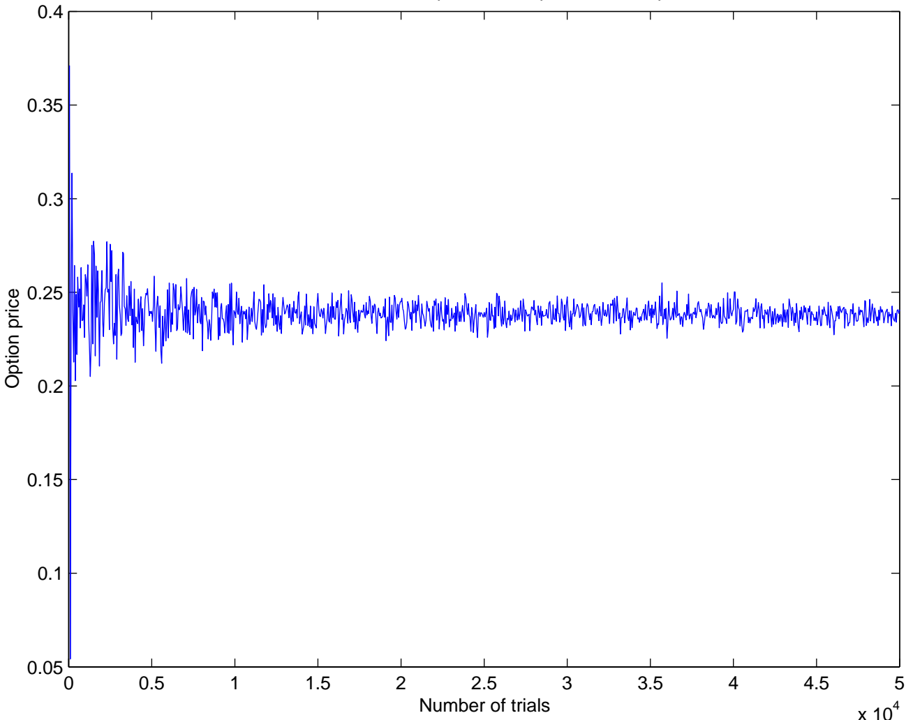
Monte Carlo calculation of the price of an option, the real price is 0.23835
