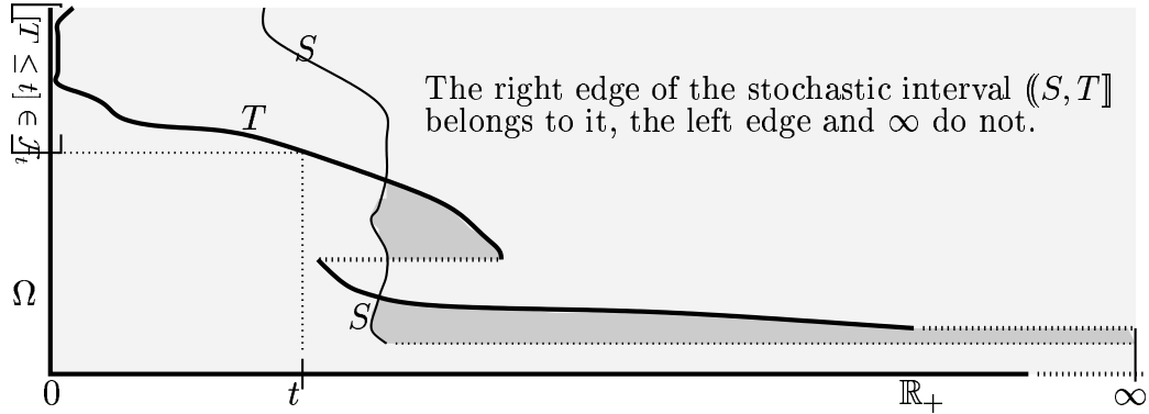
Figure 1.5 A stochastic interval
