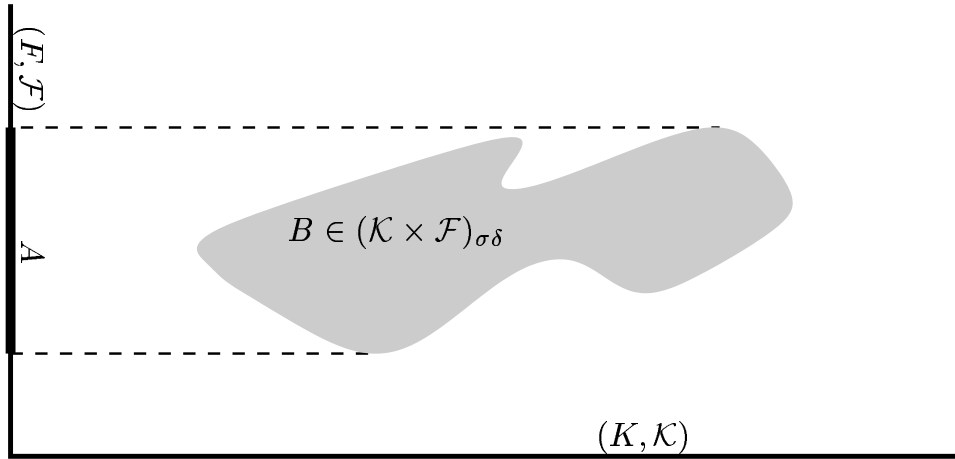
Figure A.16 An \mathcal{F} -analytic set A
