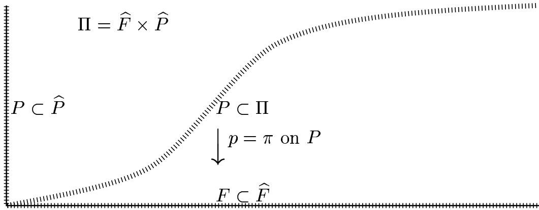
Figure A.18 Compactifying the situation
