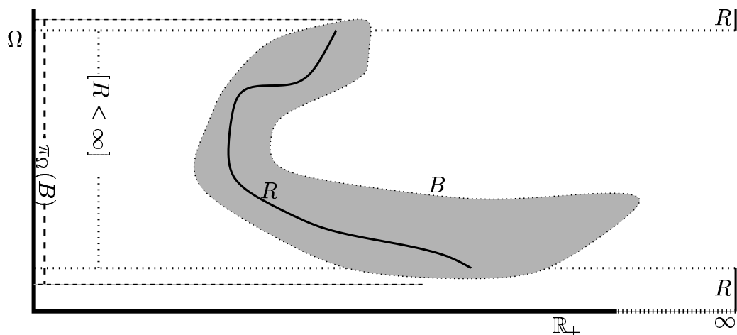
Figure A.17 The Measurable Section Theorem
