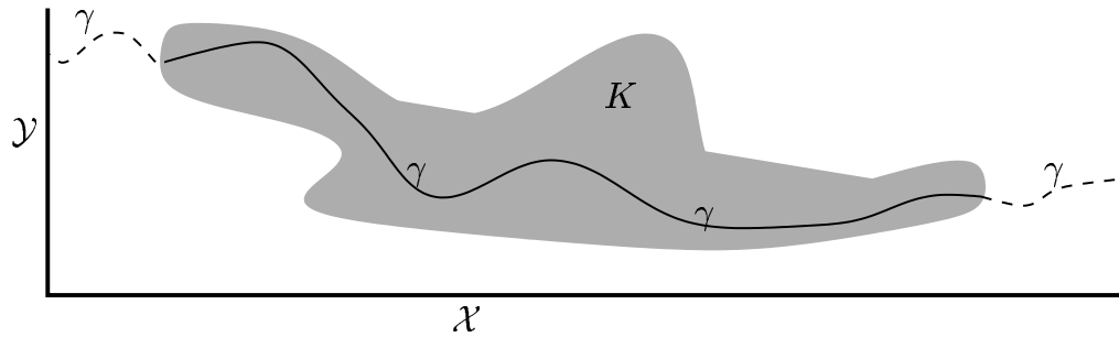
Figure A.15 The Cross Section Lemma
