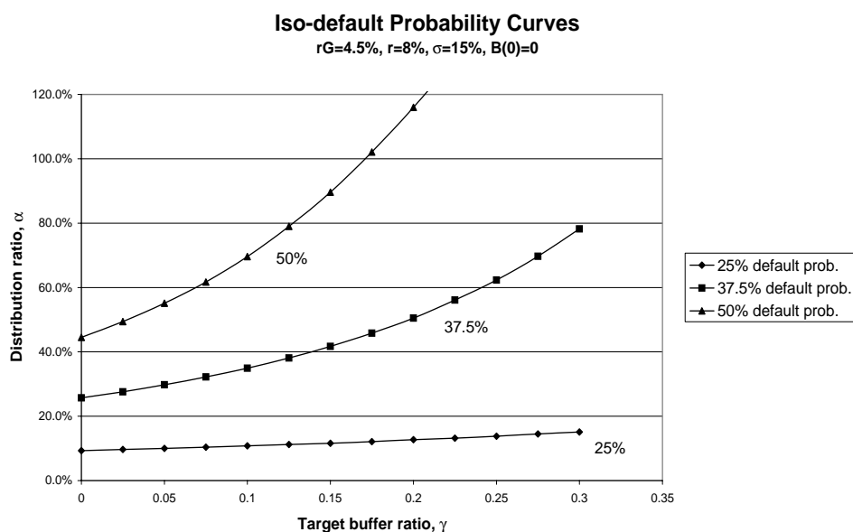
Figure 5: Iso-default probability curves
